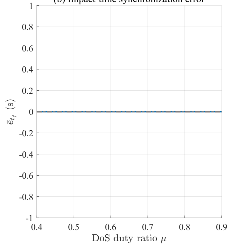
(b) Impact-time synchronization error
