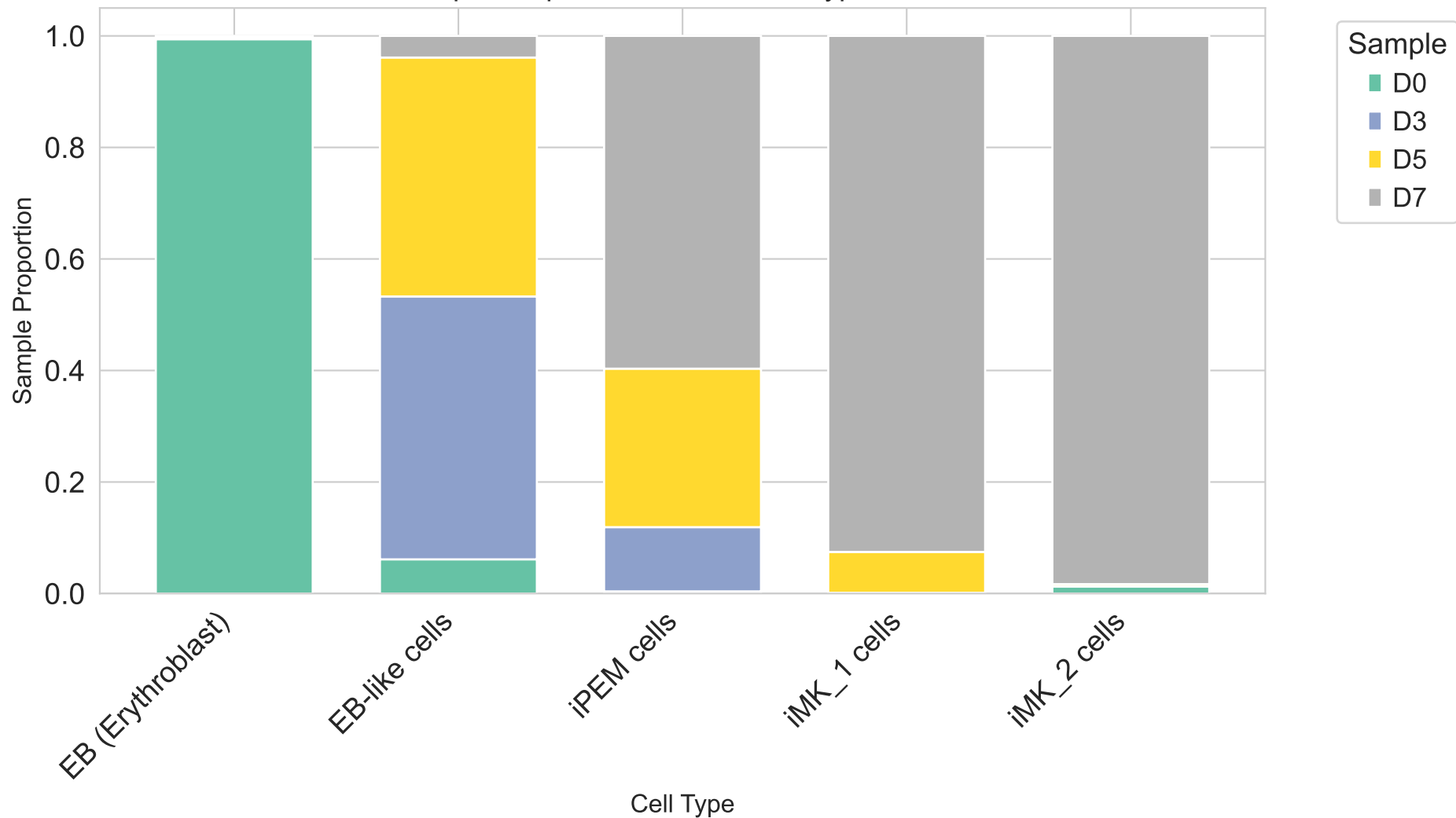
Sample Proportion in Each Cell Type Cluster
