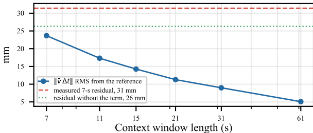
(c) The unobservable term shrinks with context, but was not learned
