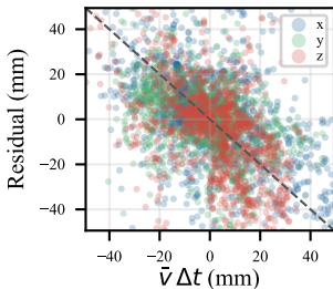
(b) 31.4 \rightarrow 26.3 mm if \tilde{\mathbf{v}} known
