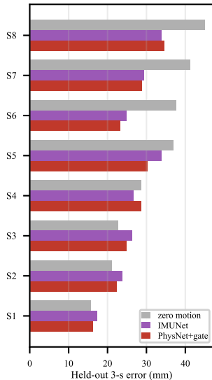
(c) Leave-one-session-out
