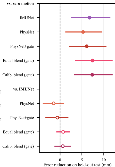
(b) Paired differences, 95% CI
