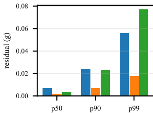
(b) Acceleration residual
