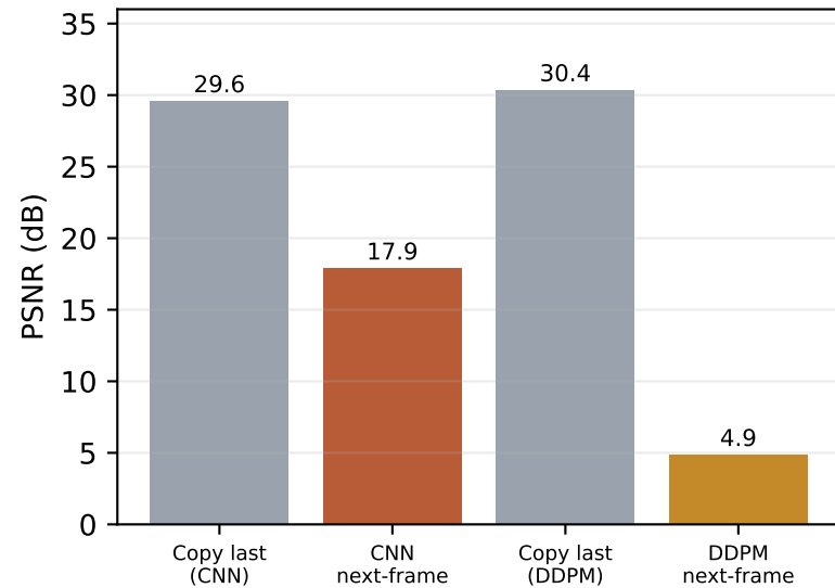
(a) Pixel generation vs copy-last
