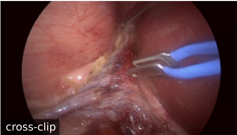
Predicted-latent retrieval
