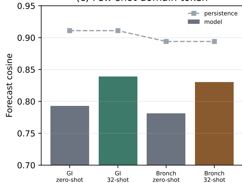
(c) Few-shot domain token
