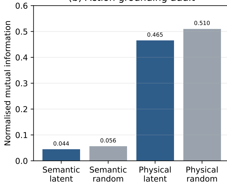
(b) Action grounding audit
