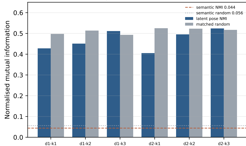
(a) Six-keyframe latent-action audit
