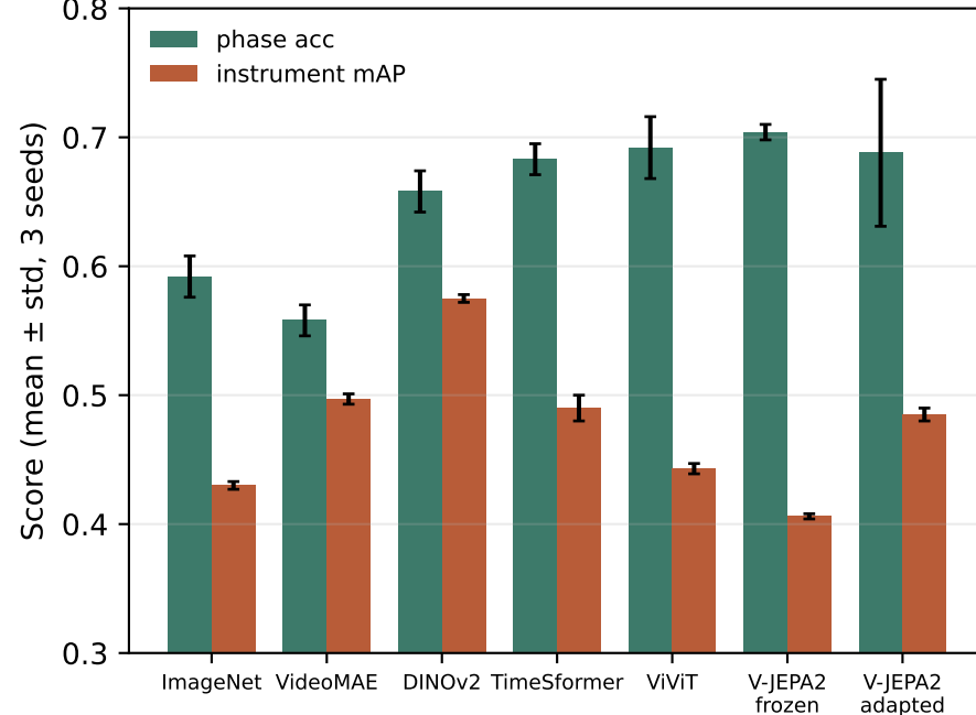
(b) Challenge-test baselines
