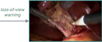
CholecT50 (laparoscopy)
