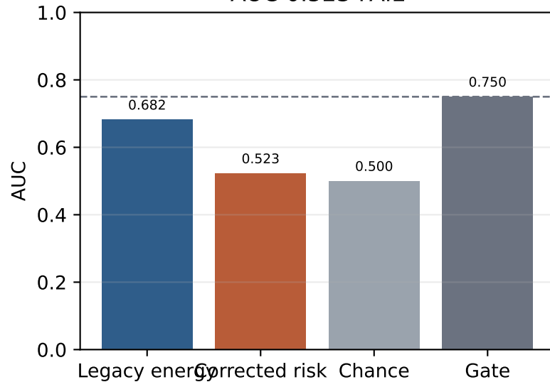
(b) Energy vs corrected risk AUC 0.523 FAIL
