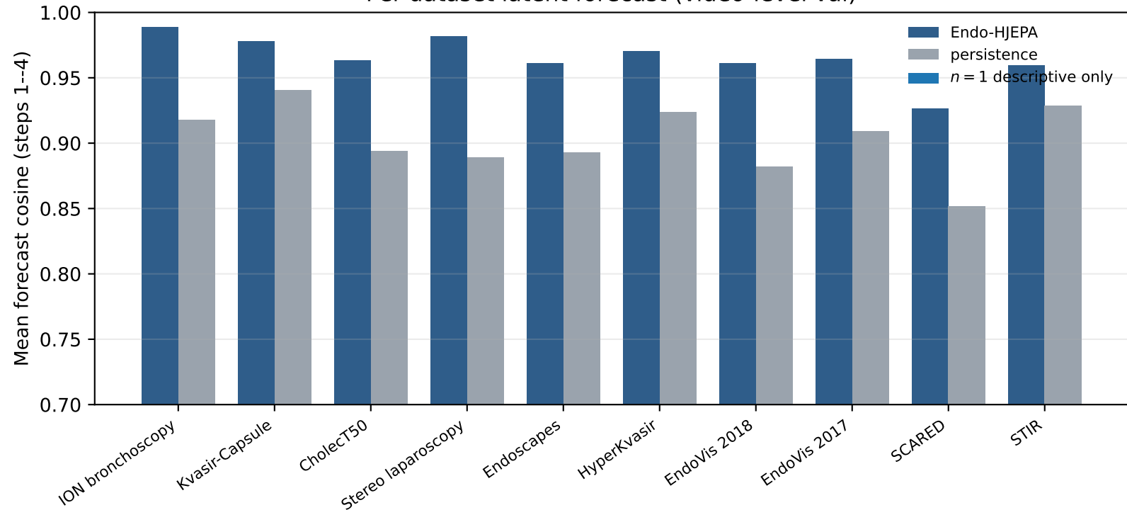
Per-dataset latent forecast (video-level val)
