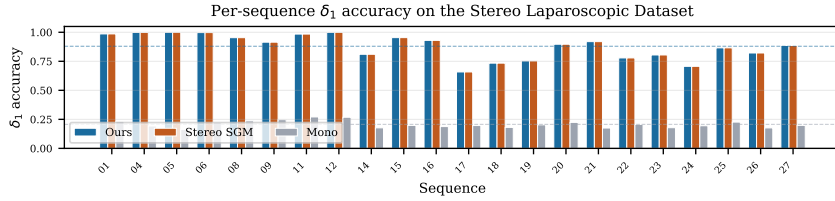
Figure 2: Per-sequence \delta_1 accuracy on the Stereo Laparoscopic Dataset (22 sequences, five endoscopes). Ours and Stereo SGM share the same SGM disparity source and therefore attain identical per-sequence depth accuracy; the heightfield contributes a per-pixel confidence map rather than a depth change. Dashed lines mark the per-method mean.
