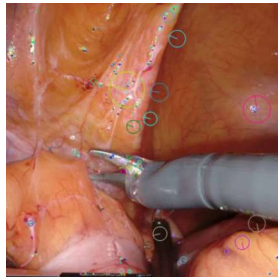
(b) Feature+attention
