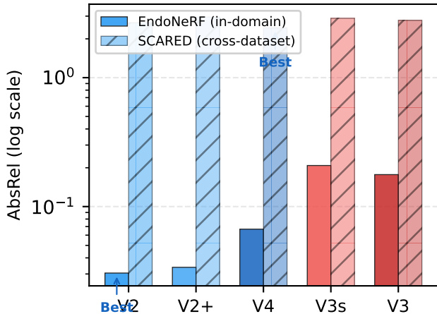
(a) Depth Accuracy
