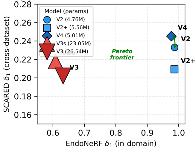
(b) In-Domain vs Cross-Dataset Trade-off
