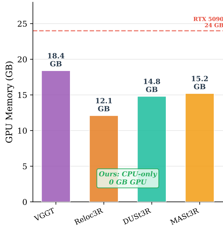
(b) GPU Memory Usage
