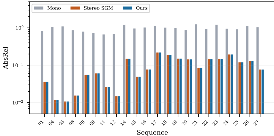
(a) Per-sequence AbsRel (identical for Ours and SGM)
