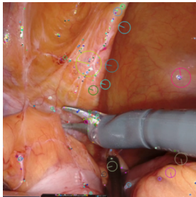
(b) Feature+attention
