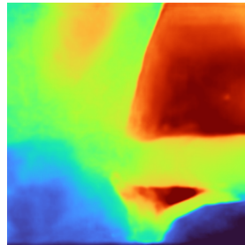
(e) Heightfield
