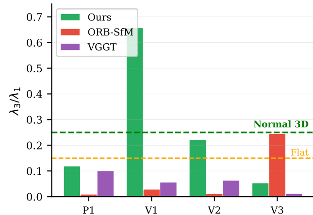
(a) 3D shape ratio
