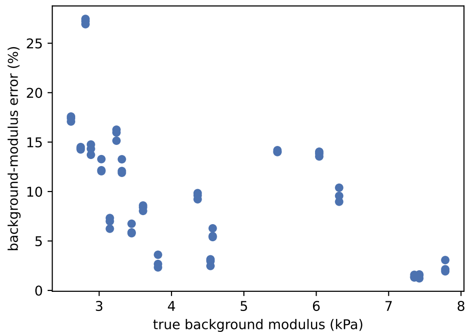
Error versus stiffness
