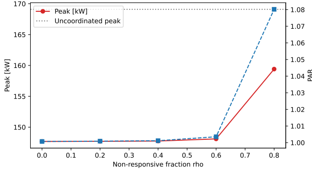
FIGURE 2. Aggregate peak and PAR versus the non-responsive fraction \rho . The horizontal axis labelled “rho” in the plotted image denotes this fraction \rho , not the ADMM penalty \rho_{ADMM} .
