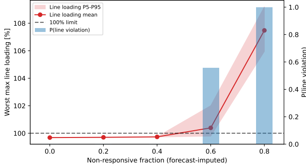
FIGURE 4. Monte-Carlo forecast-uncertainty sweep (200 draws per fraction). Worst maximum line loading mean with its P5–P95 band versus the non-responsive fraction \rho (left axis, with the 100% thermal limit), and the probability of a line violation as bars (right axis). The image’s “rho” axis is the non-responsive fraction \rho .
