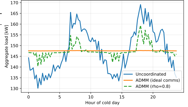
FIGURE 1. Aggregate cold-day load: uncoordinated double-peak versus the flat ADMM ideal profile ( \approx 147.7 kW) and the \varrho = 0.8 imputed case with residual peaks. Here \varrho is the non-responsive fraction.
