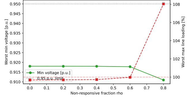
FIGURE 3. Worst minimum bus voltage (left axis) and worst maximum line loading (right axis) versus the non-responsive fraction \varrho — the headline feasibility figure. Line loading clears below 100% through \varrho = 0.6 and re-violates at \varrho = 0.8 . The image’s “rho” axis is the non-responsive fraction \varrho .
