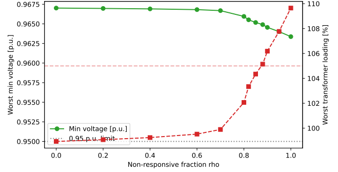
FIGURE 5. Worst minimum bus voltage (left axis) and worst maximum transformer loading (right axis) versus the non-responsive fraction \rho — the headline feasibility figure. Loading stays cleared below the 105% limit through \rho = 0.85 , crosses it near \rho = 0.87 (violated by \rho = 0.88 ), and ramps to the uncoordinated 109.6% at \rho = 1 . The image’s “rho” axis is the non-responsive fraction \rho .
