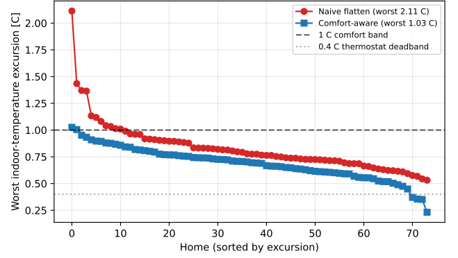
FIGURE 2. Per-home worst modelled indoor-temperature excursion from setpoint, comfort-aware coordination ( \gamma = 2 ) versus a naive energy-only flatten, propagated through each home’s RC thermal model. The comfort-aware worst is 1.03^\circ\text{C} (median 0.70^\circ\text{C} ) against 2.11^\circ\text{C} for the energy-only case; the 1^\circ\text{C} comfort band and the 0.4^\circ\text{C} thermostat deadband are marked.
