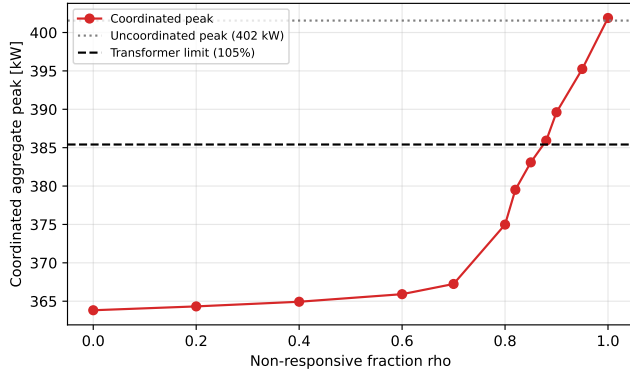
FIGURE 3. Coordinated aggregate peak versus the non-responsive fraction \varrho , against the uncoordinated level and the peak that corresponds to the transformer thermal limit. The horizontal axis labelled “rho” in the plotted image denotes this fraction \varrho , not the ADMM penalty \rho_{\text{ADMM}} .
