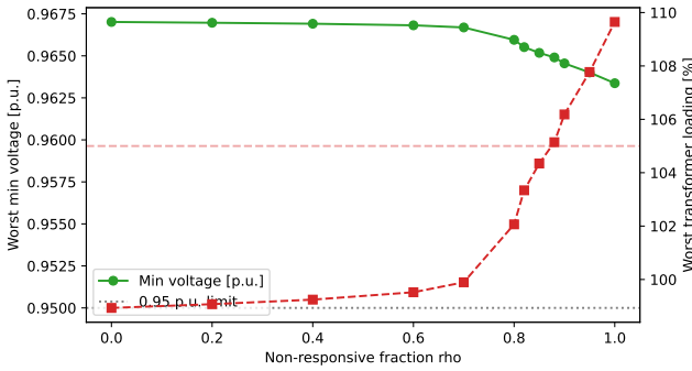
FIGURE 7. Worst minimum bus voltage (left axis) and worst maximum transformer loading (right axis) versus the non-responsive fraction \rho , the headline feasibility figure. Loading stays cleared below the 105% limit through \rho = 0.85 , crosses it near \rho = 0.87 (violated by \rho = 0.88 ), and ramps to the uncoordinated 109.6% at \rho = 1 . The image's "rho" axis is the non-responsive fraction \rho .
