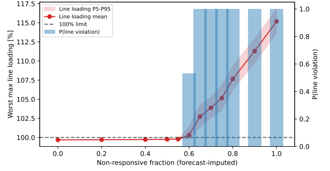
FIGURE 4. Monte-Carlo forecast-uncertainty sweep (200 draws per fraction). Worst maximum line loading mean with its P5–P95 band versus the non-responsive fraction \varrho (left axis, with the 100% thermal limit), and the probability of a line violation as bars (right axis). The image's "rho" axis is the non-responsive fraction \varrho .
