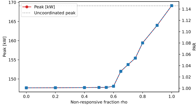
FIGURE 2. Aggregate peak and PAR versus the non-responsive fraction \rho . The horizontal axis labelled “rho” in the plotted image denotes this fraction \rho , not the ADMM penalty \rho_{\text{ADMM}} .
