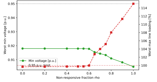
FIGURE 3. Worst minimum bus voltage (left axis) and worst maximum line loading (right axis) versus the non-responsive fraction \rho — the headline feasibility figure. Loading stays cleared below 100% through \rho = 0.6 , crosses the limit near \rho = 0.62 , and ramps linearly to the uncoordinated 115% at \rho = 1 . The image’s “rho” axis is the non-responsive fraction \rho .
