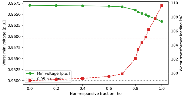
FIGURE 5. Worst minimum bus voltage (left axis) and worst maximum transformer loading (right axis) versus the non-responsive fraction \rho — the headline feasibility figure. Loading stays cleared below the 105% limit through \rho = 0.85 , crosses it near \rho = 0.87 (violated by \rho = 0.88 ), and ramps to the uncoordinated 109.6% at \rho = 1 . The image’s “rho” axis is the non-responsive fraction \rho .
