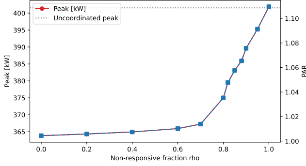
FIGURE 3. Aggregate peak and PAR versus the non-responsive fraction \rho . The horizontal axis labelled “rho” in the plotted image denotes this fraction \rho , not the ADMM penalty \rho_{\text{ADMM}} .
