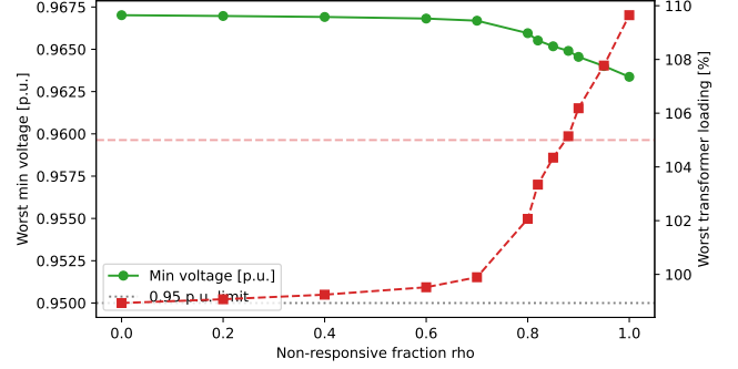
FIGURE 6. Worst minimum bus voltage (left axis) and worst maximum transformer loading (right axis) versus the non-responsive fraction \varrho — the headline feasibility figure. Loading stays cleared below the 105% limit through \varrho = 0.85 , crosses it near \varrho = 0.87 (violated by \varrho = 0.88 ), and ramps to the uncoordinated 109.6% at \varrho = 1 . The image’s “rho” axis is the non-responsive fraction \varrho .
