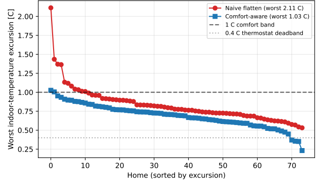
FIGURE 3. Per-home worst modelled indoor-temperature excursion from setpoint, comfort-aware coordination ( \gamma = 2 ) versus a naive energy-only flatten, propagated through each home’s RC thermal model. The comfort-aware worst is 1.03 °C (median 0.70 °C) against 2.11 °C for the energy-only case; the 1 °C comfort band and the 0.4 °C thermostat deadband are marked.
