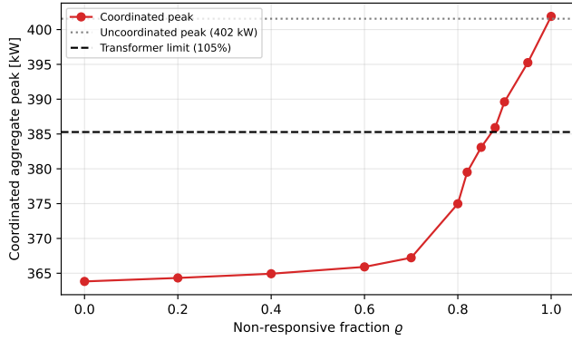
FIGURE 5. Coordinated aggregate peak versus the non-responsive fraction \rho , against the uncoordinated level and the peak that corresponds to the transformer thermal limit.
