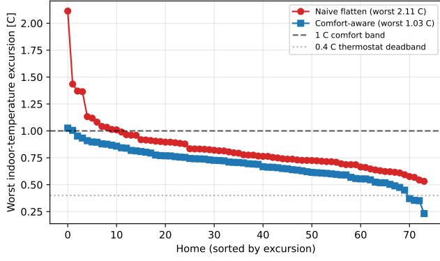
FIGURE 4. Per-home worst modelled indoor-temperature excursion from setpoint, comfort-aware coordination ( \gamma = 2 ) versus a naive energy-only flatten, propagated through each home's RC thermal model. The comfort-aware worst is 1.03^\circ\text{C} (median 0.70^\circ\text{C} ) against 2.11^\circ\text{C} for the energy-only case; the 1^\circ\text{C} comfort band and the 0.4^\circ\text{C} thermostat deadband are marked.
