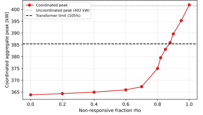
FIGURE 3. Coordinated aggregate peak versus the non-responsive fraction \varrho , against the uncoordinated level and the peak that corresponds to the transformer thermal limit. The horizontal axis labelled “rho” in the plotted image denotes this fraction \varrho , not the ADMM penalty \rho_{\text{ADMM}} .
