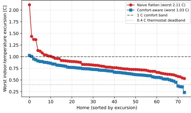
FIGURE 2. Per-home worst modelled indoor-temperature excursion from setpoint, comfort-aware coordination ( \gamma = 2 ) versus a naive energy-only flatten, propagated through each home's RC thermal model. The comfort-aware worst is 1.03^\circ\text{C} (median 0.70^\circ\text{C} ) against 2.11^\circ\text{C} for the energy-only case; the 1^\circ\text{C} comfort band and the 0.4^\circ\text{C} thermostat deadband are marked.
