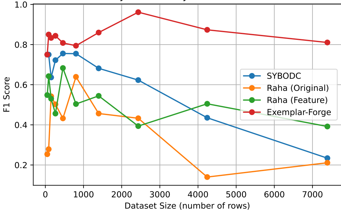
Accuracy Consistency Across Dataset Sizes
