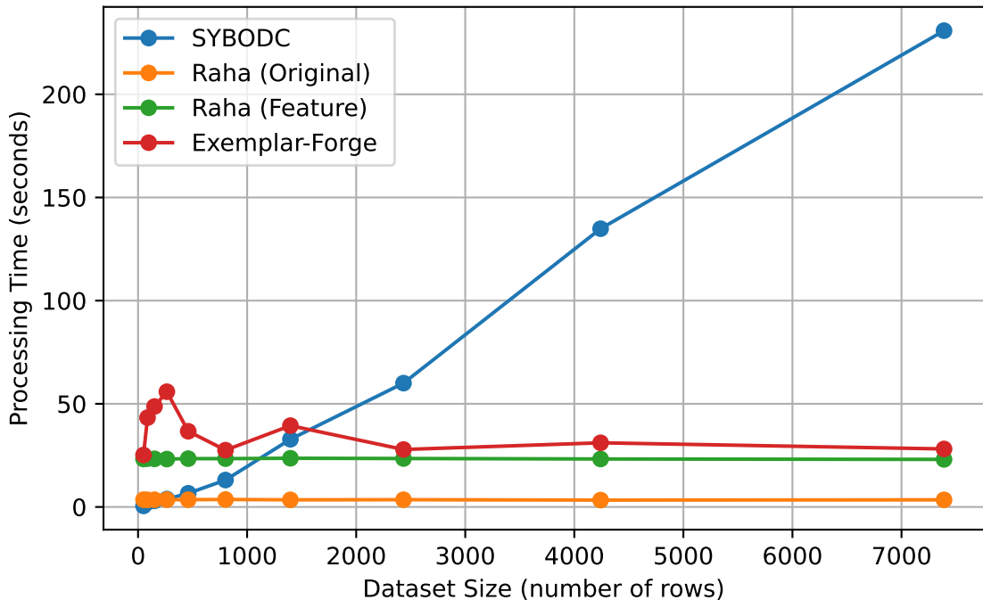
Computational Scalability: Dataset Size vs Processing Time
