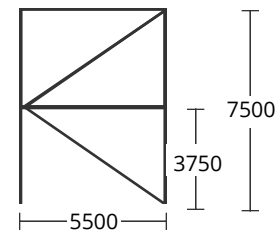
TRUSS PILLAR
