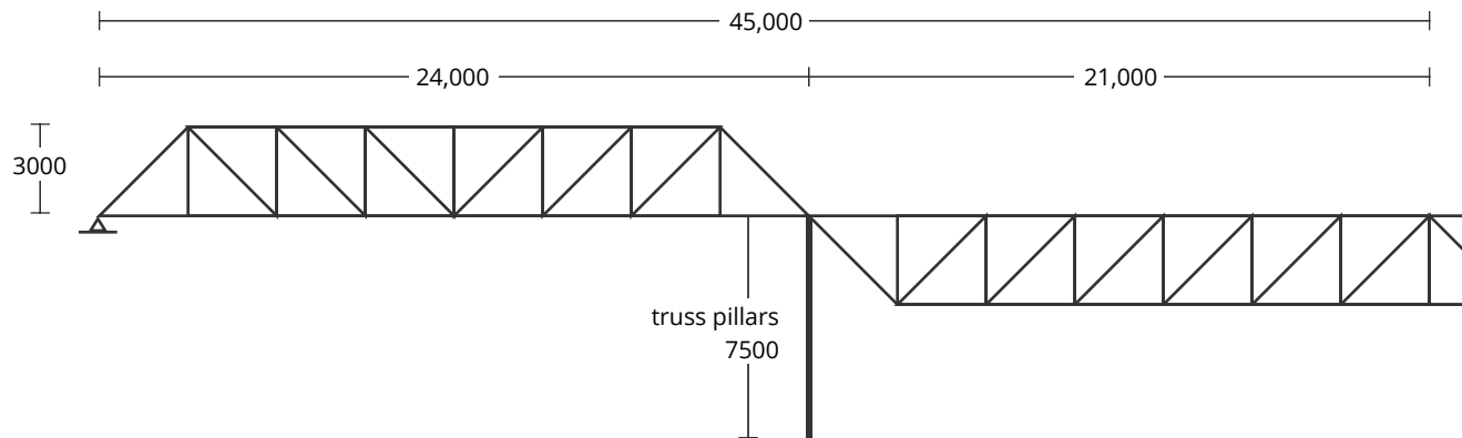
SIDE ELEVATION
