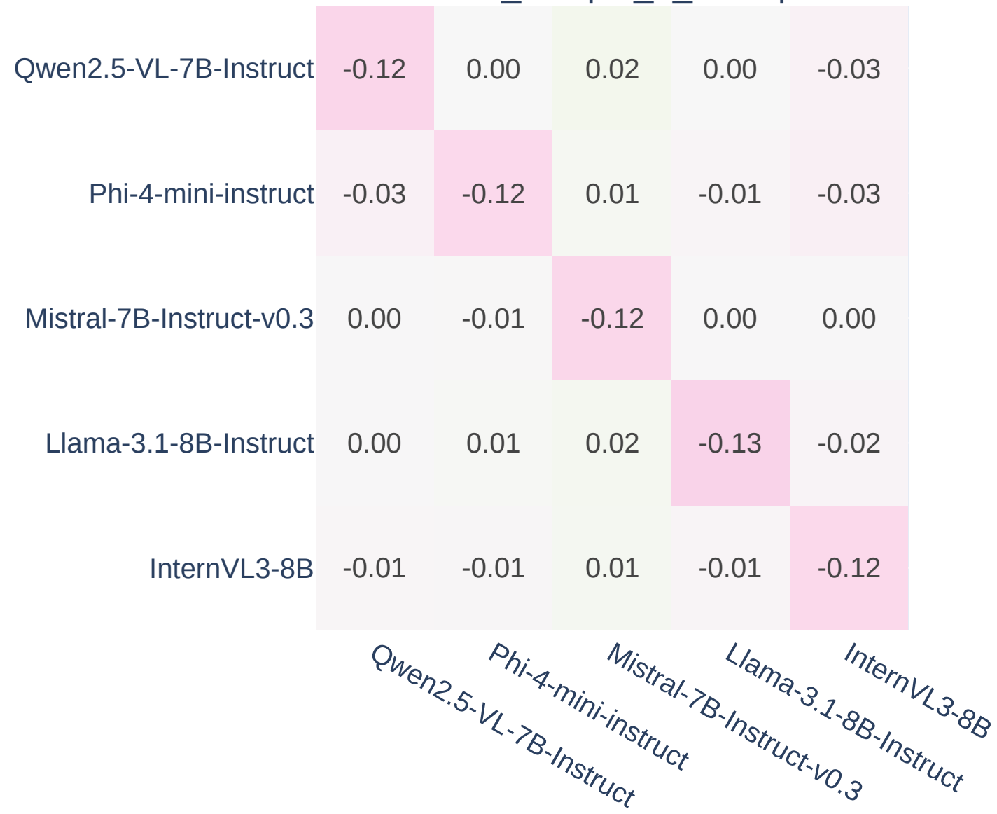
random_sample_5_examples
