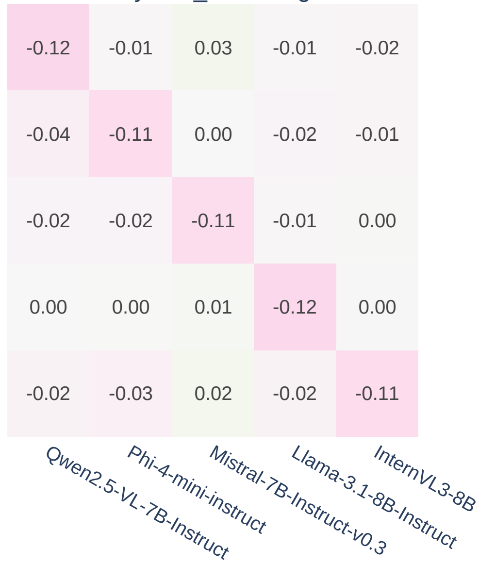
stylistic_clustering
