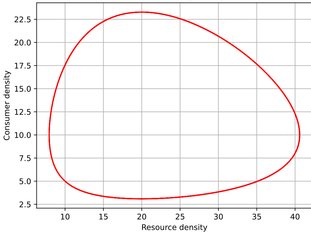
Consumer-Resource phase portrait
