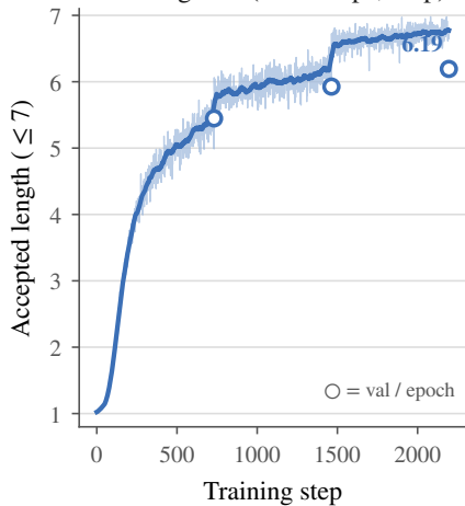
Convergence (2196 steps, 3 ep)
