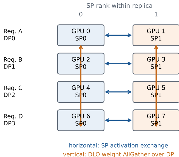
(a) DP4 x SP2 process grid
