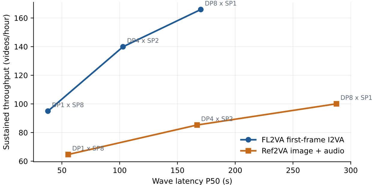
Conditioning path changes scale, not the Pareto direction
