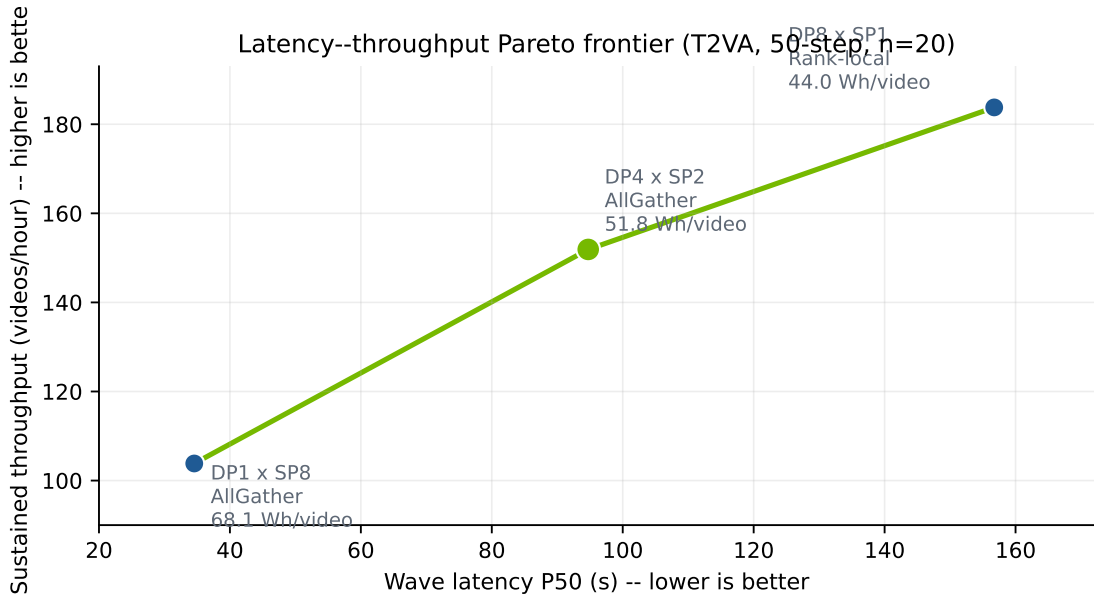
Figure 1: T2VA latency–throughput frontier. Labels include measured eight-GPU board energy per output.
