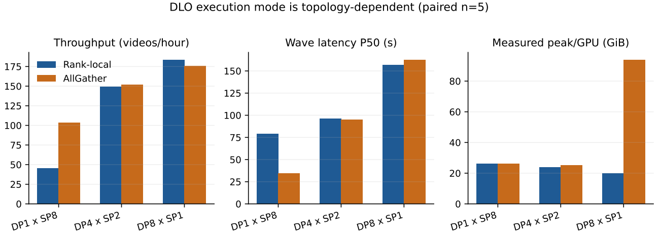
Figure 2: Paired DLO-mode comparison. AllGather’s benefit reverses at DP8.
