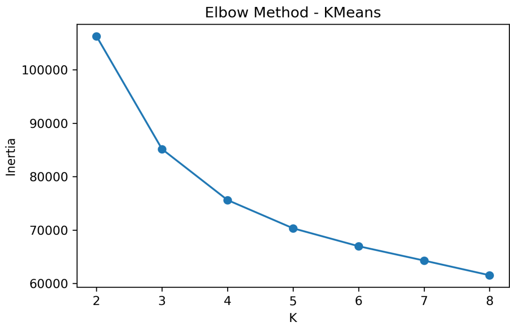
Figura 3: Elbow Method KMeans
