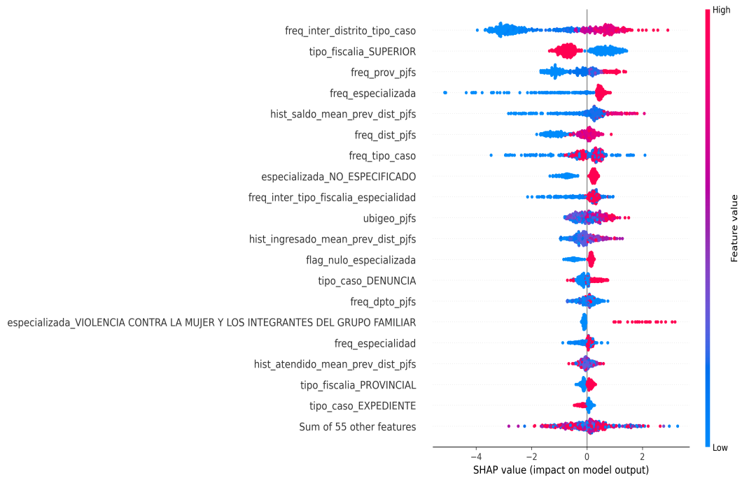
Figura 1: SHAP Beeswarm - Top 20 features
