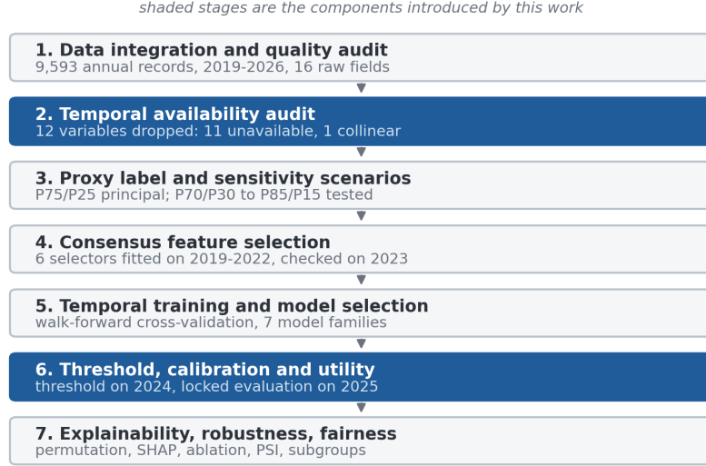
Fig. 1 Stages of the proposed framework. The framework extends a conventional predictive pipeline with explicit temporal availability auditing, role-separated temporal evaluation, and joint assessment of discrimination, calibration and decision utility. The availability audit is repeated after feature selection so that the final fitted matrix, rather than only the intended exclusion rule, determines the audit outcome.
