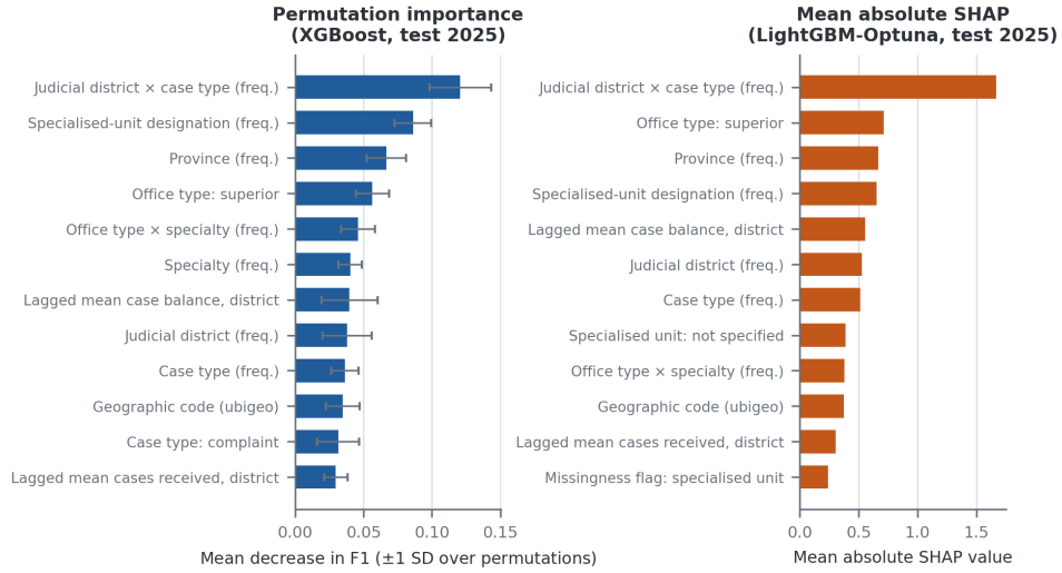
Fig. 9 Global variable importance under two attribution methods. Left: permutation importance on the reported XGBoost model, with error bars giving \pm 1 SD over permutations. Right: mean absolute SHAP values on the tuned LightGBM configuration. The two attributions were computed on different estimators and are shown separately for that reason. Variables carry readable labels; Additional file 3 maps each label to the exact column name in the pipeline.
