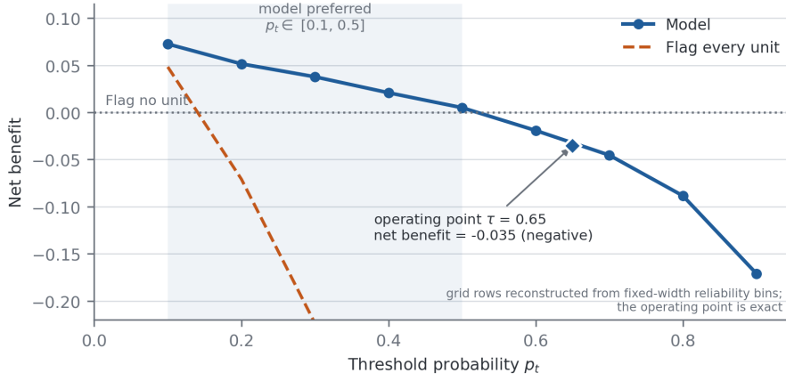
Fig. 8 Decision curve analysis on the 2025 evaluation set. The model exceeds both default strategies for threshold probabilities between 0.1 and 0.5. At the F1-optimal operating point \tau = 0.65 its net benefit is negative, meaning that flagging no unit would be preferable for a decision maker holding that threshold. The grid is reconstructed from fixed-width reliability bins; only the operating point is computed from the exact confusion matrix.
