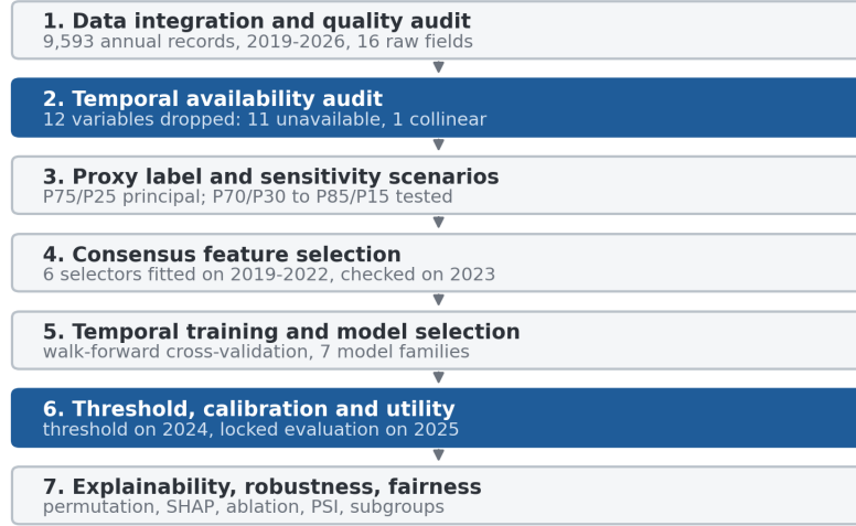
Fig. 1 Stages of the proposed framework. The framework extends a conventional predictive pipeline with explicit temporal availability auditing, role-separated temporal evaluation, and joint assessment of discrimination, calibration and decision utility. The availability audit is repeated after feature selection so that the final fitted matrix, rather than only the intended exclusion rule, determines the audit outcome.
