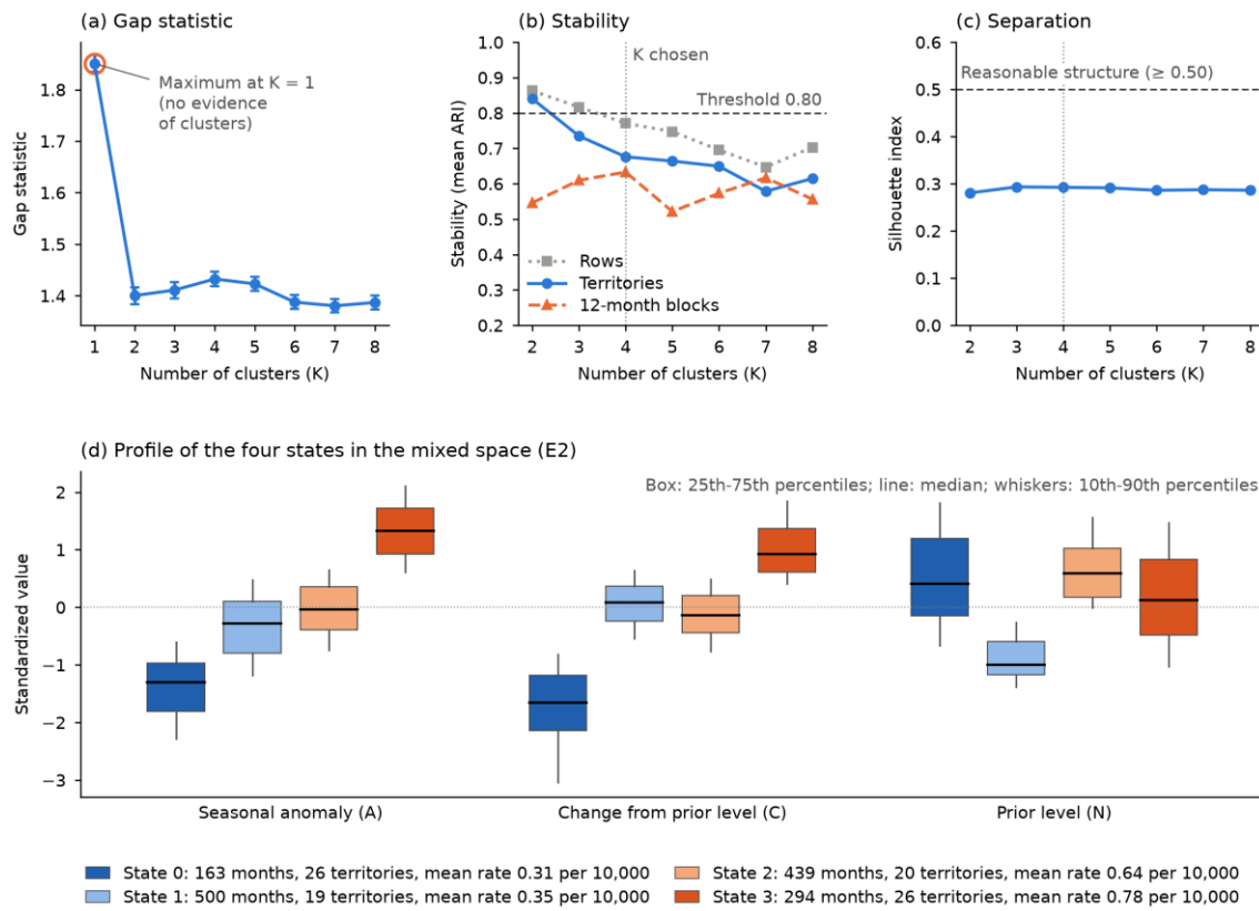
Fig. 5. Diagnostics and state profiles in E2, 2019–2023 (n = 1,396 territory-months). (a) Gap statistic. (b) ARI stability. (c) Silhouette. (d) Standardized features.
