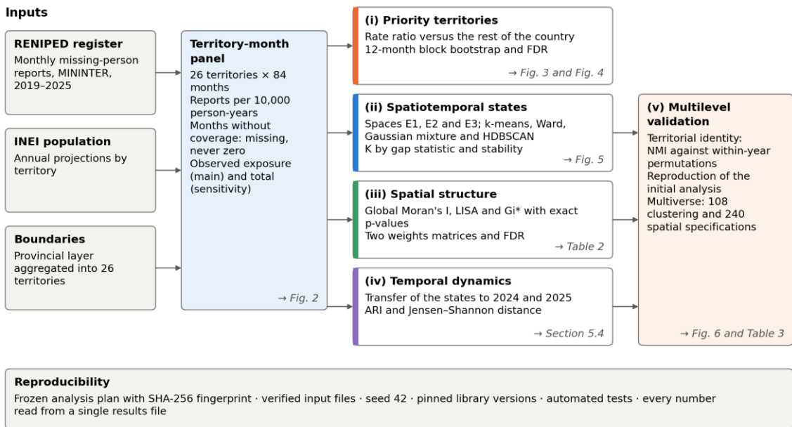
Fig. 1. Architecture of the GeoAI framework: sources, territory-month panel, analytical stages and validation. Italic arrows indicate the section where each result is reported.
