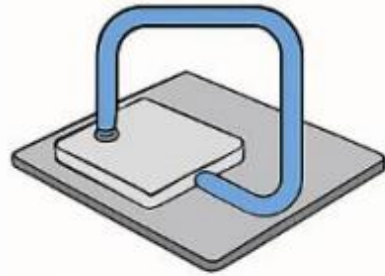
Single-Phase DLC(SPDLCL)
