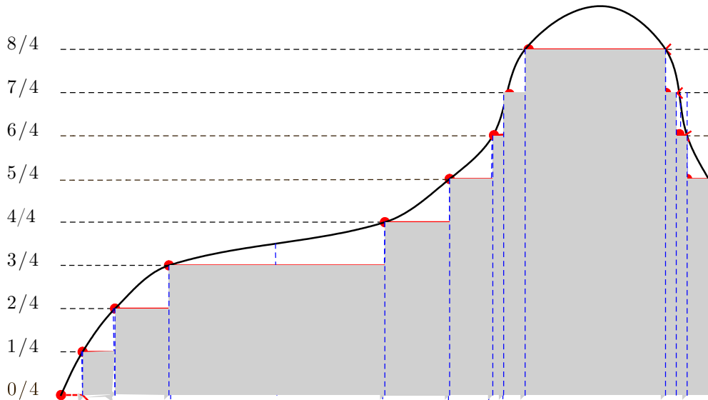
Figure 20.7. f apprimated by f_2
