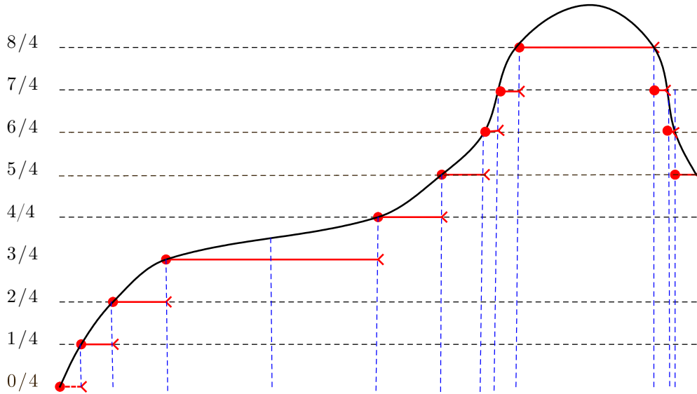
Figure 20.6. f approximated by f_2
