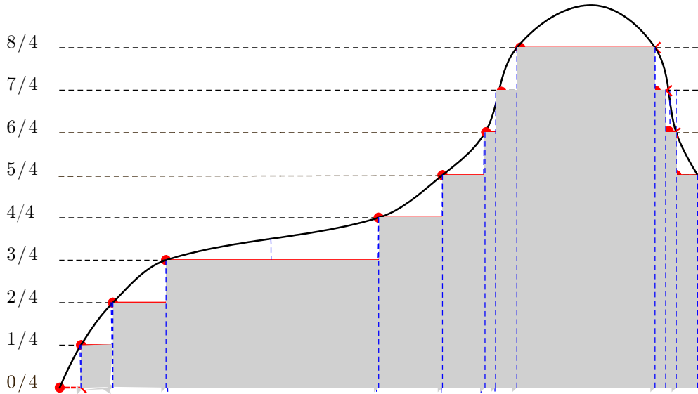
Figure 21.7. f approximated by f_2
