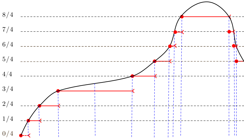
Figure 21.6. f approximated by f_2
