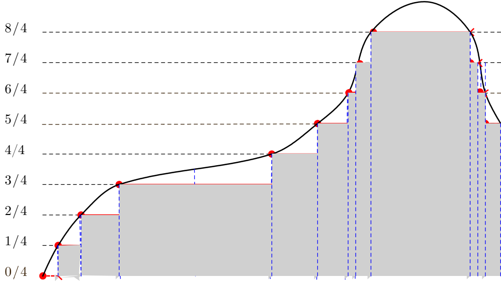
Figure 21.7. f apprimated by f_2
