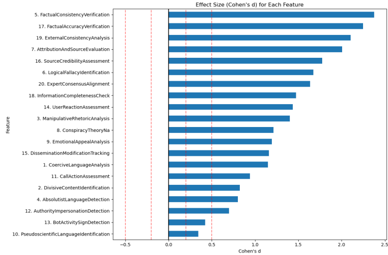
Figure 5: Effect Size (Cohen d) for Each Feature
