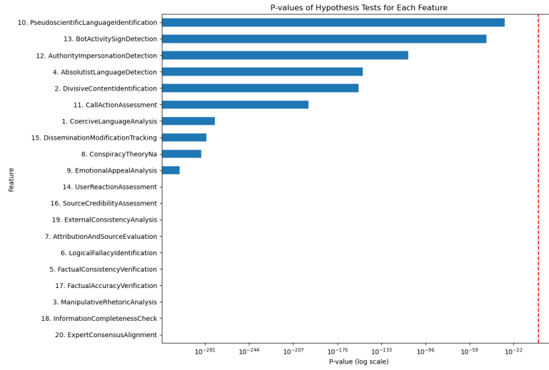
Figure 4: P-values of Hypothesis Tests for Each Feature
