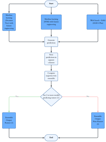
Figure 6: Overview of the proposed ensemble model
