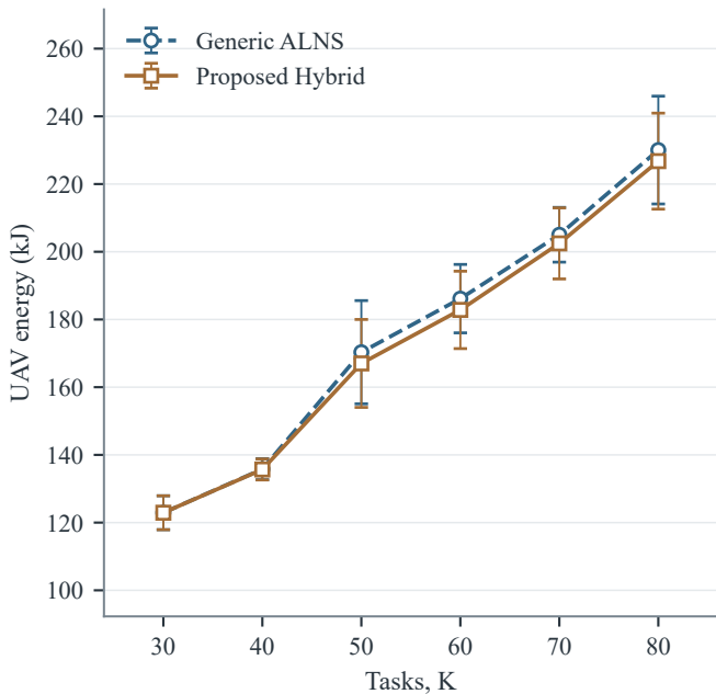
(a) Energy versus workload
