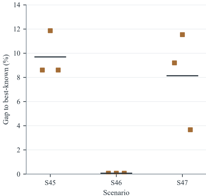
(a) Standard-search quality
