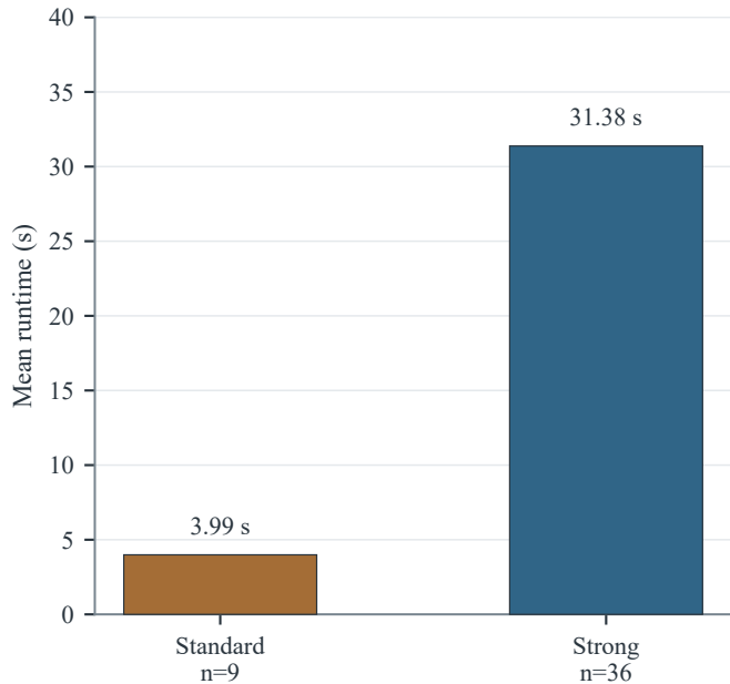
(b) Search cost
